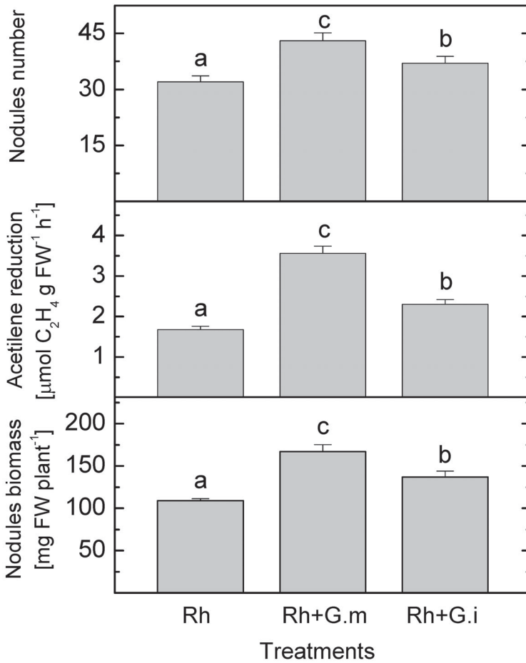
Figure 1. Nodule number, biomass and nitrogenase activity in inoculated pea plants at low phosphorus level ( 60\text{mg P}_2\text{O}_5 \text{ kg soil}^{-1} ). Values are means \pm SE, n = 3 ; different letters indicate significant differences assessed by Fisher LSD test ( P \leq 0.05 ) after performing ANOVA multifactor analysis.
